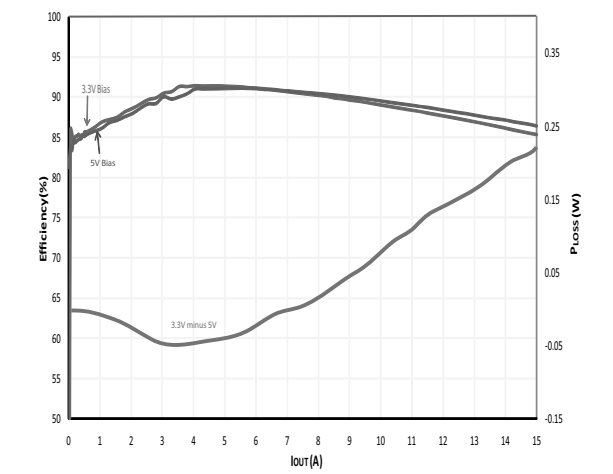
Efficiency/Power Loss-P-Save (V OUT = 1.5 V, V IN = 12 V, SiC401B)
